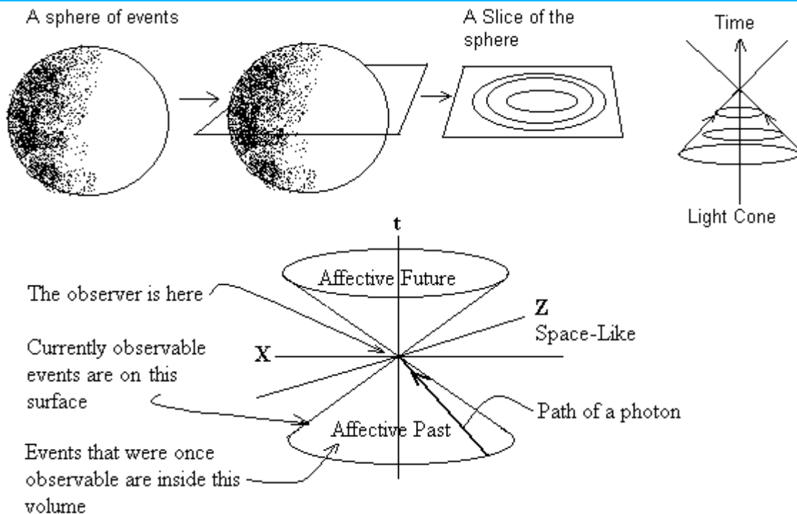
A Slice of a Sphere of Events Represented by a Light Cone (Solution of 0 = x^2 + z^2 - (ct)^2 )
